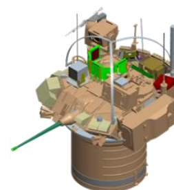
Figure C-3. Manned turret
