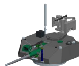
Figure C-4. Unmanned turret
